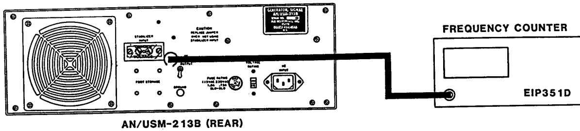
REAR PANEL SET UP
